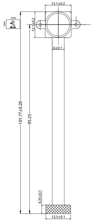
TOP VIEW
