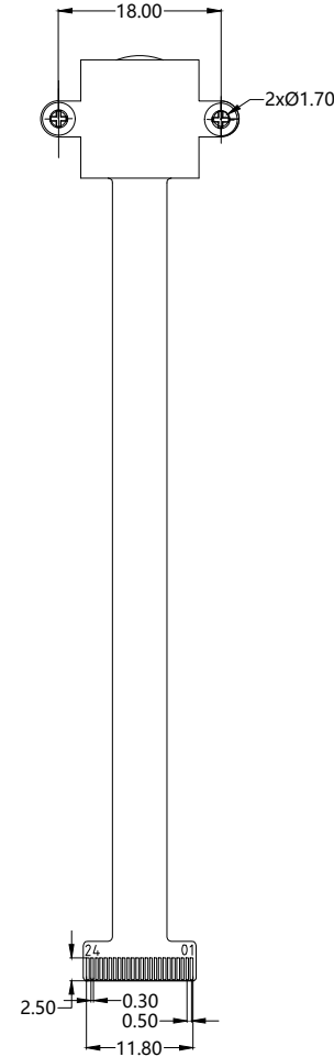
BOTTOM VIEW
